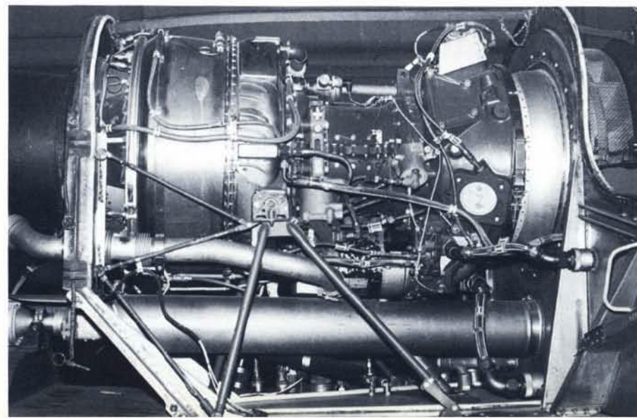
(Right) The UH-1C was initially powered by a Lycoming T-53-L-9 engine and later with the 1,100 shp T-53-11 engine. These more powerful engines required a larger vertical fin and synchronized elevators to compensate for the increased torque. (Bell)
