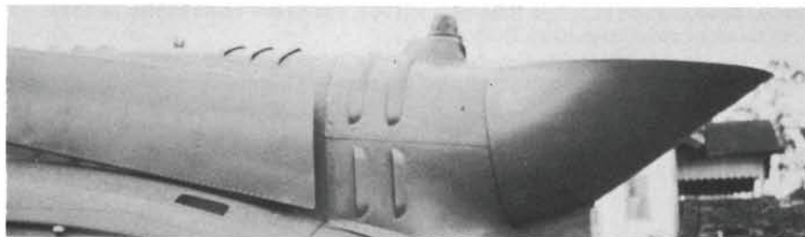
(Above) The engine heat baffle and 'toilet bowl' exhaust comprised the IR suppressor kit. (Koenig via Pete Harlem)
