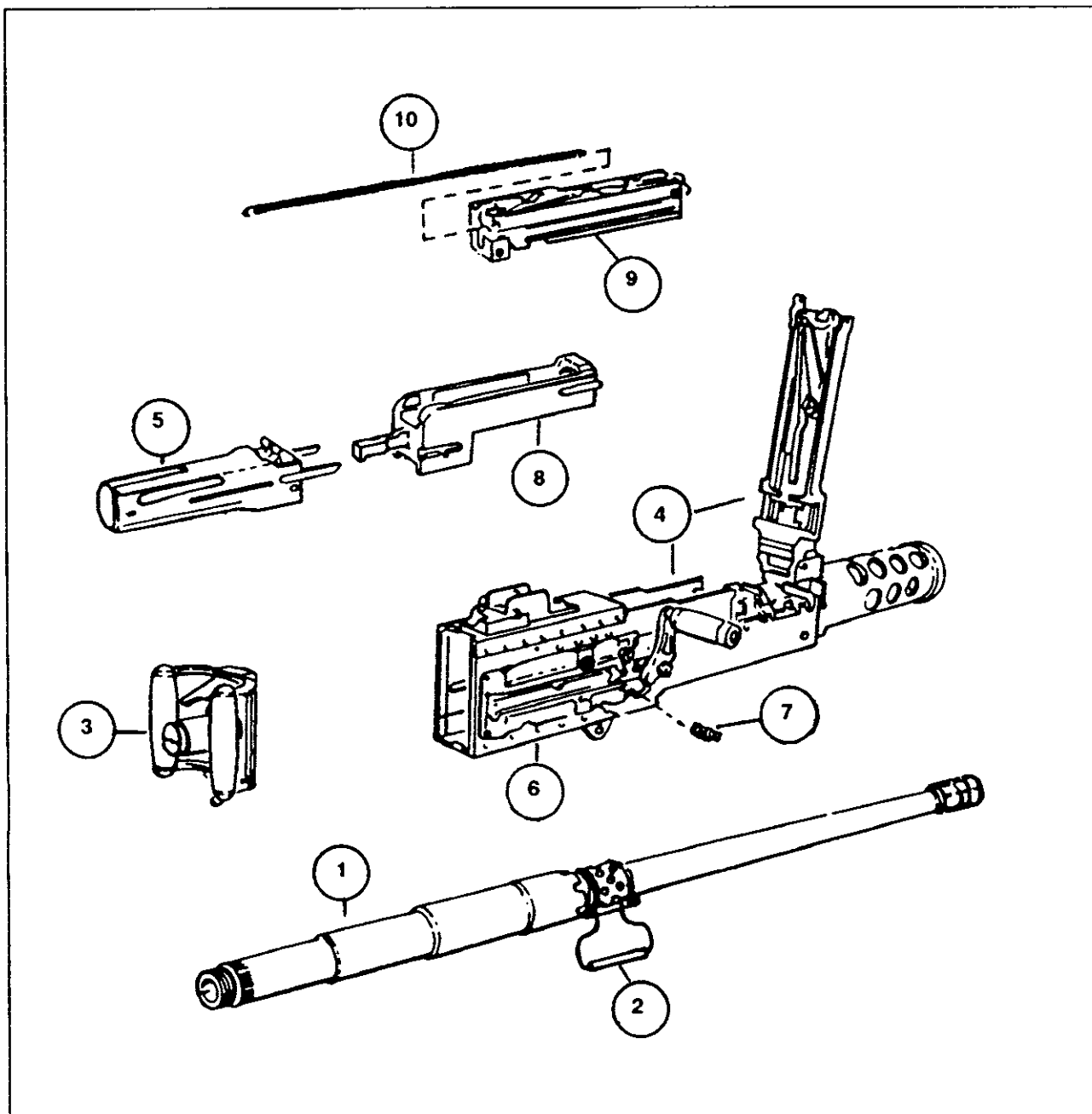
Figure 1-5. Components of the caliber .50 MG.
