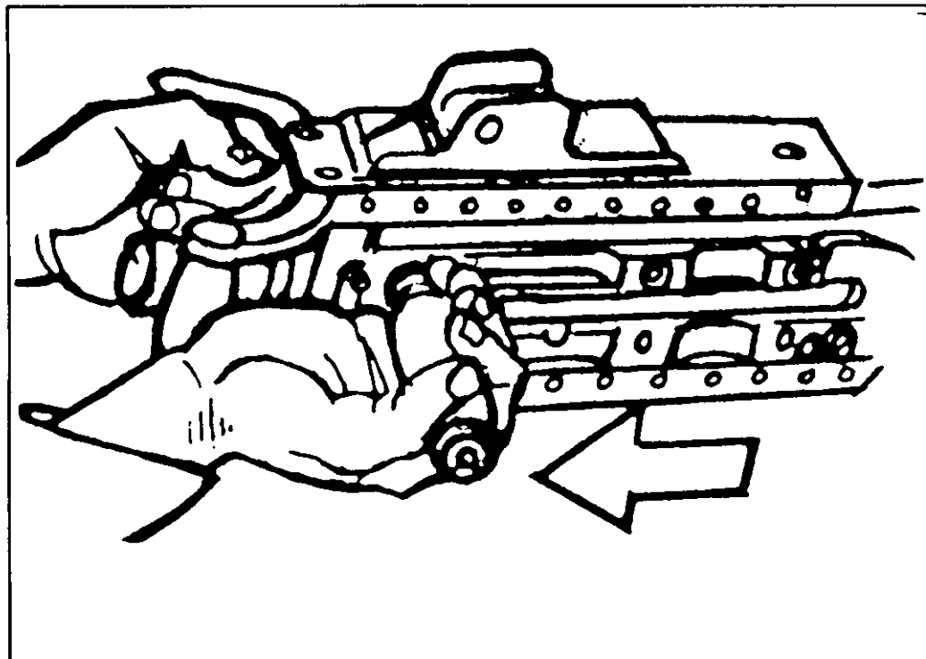
Figure 3-20. Releasing the bolt.
