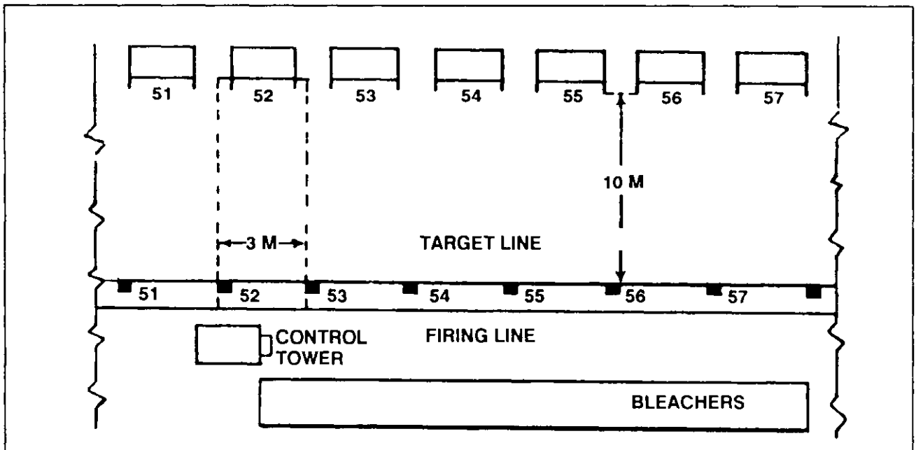
Figure C-2. Ten-meter range layout.
