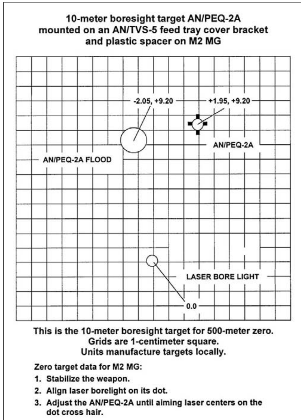
Figure G-12. Alignment of M2 with the AN/PEQ-2A.
