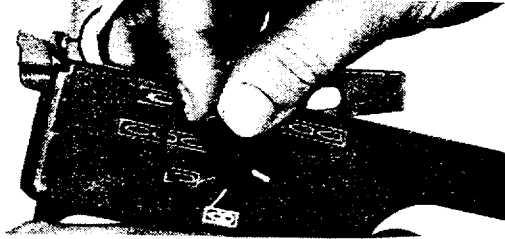
Ill.# 34A - Rotating the safety/selector lever clockwise
