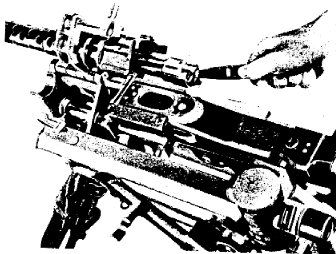
Figure 42 — Removing a Hot Barrel
