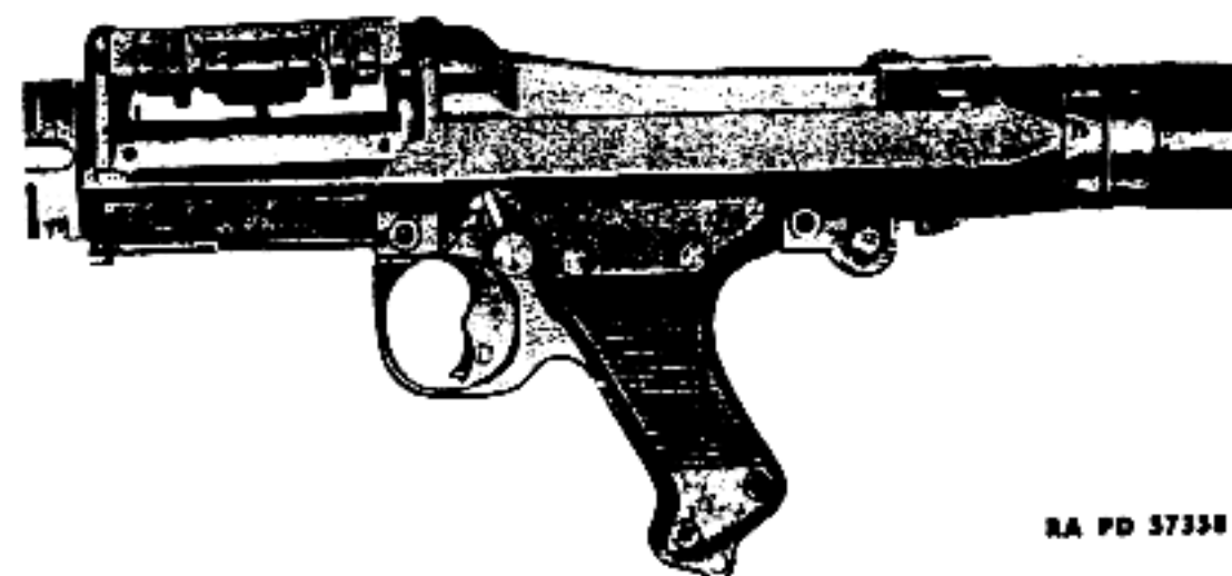
Figure 31 — Safety at Safe — Letter "S," Uncovered
