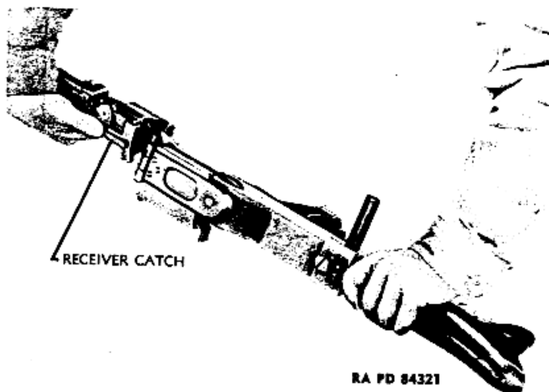
Figure 39 — Unlocking and Rotating Receiver
