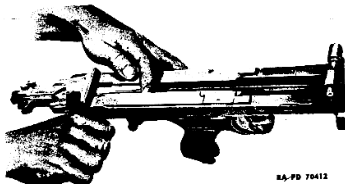
Figure 49 — Removal of Bolt
