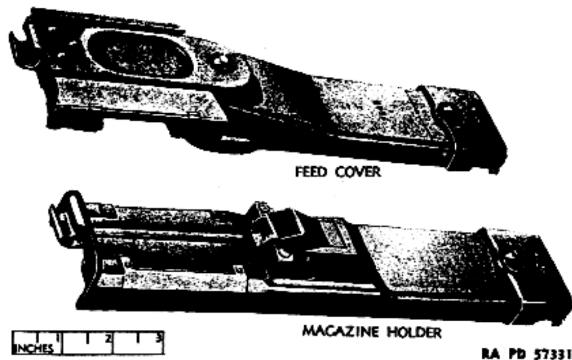
Figure 23 — Feed Cover and Magazine Holder — Top View
