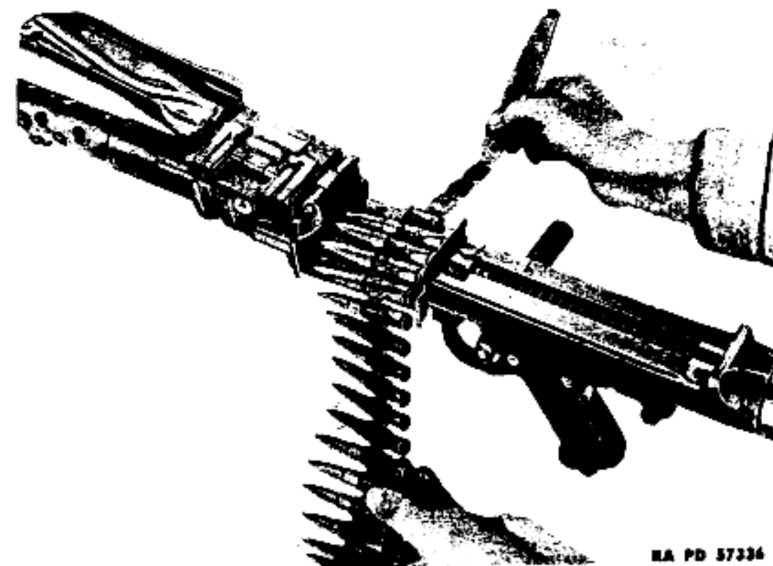
Figure 19 — Positioning Belt on Feed Block
