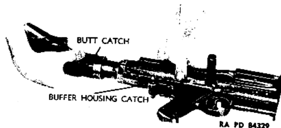
Figure 46 — German 7.9-mm Dual Purpose Machine Gun MG34 — Removal of Butt
