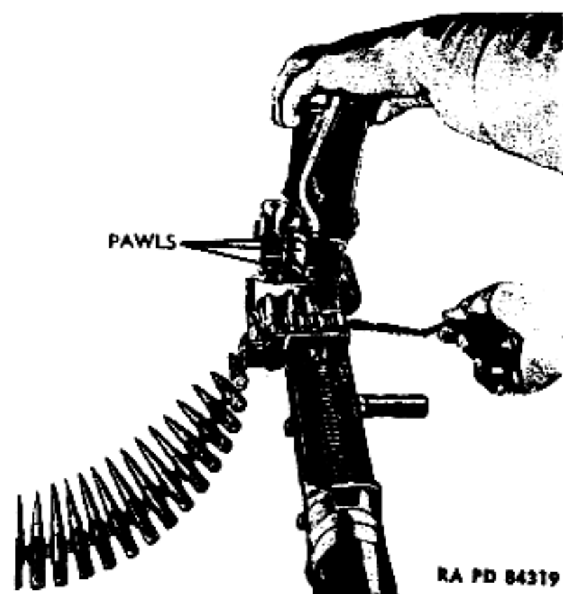
Figure 20 - Closing of Feed Cover
