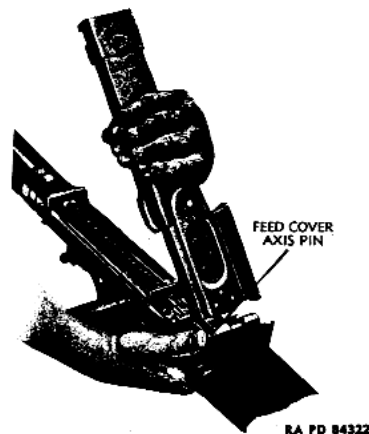
Figure 25 — Removal of Feed Cover
