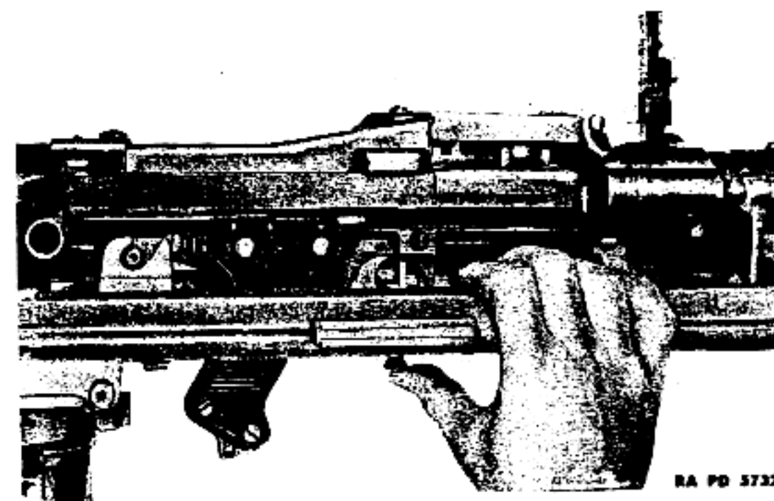
Figure 32 — Adjustment of Trigger Finger for Single Fire
