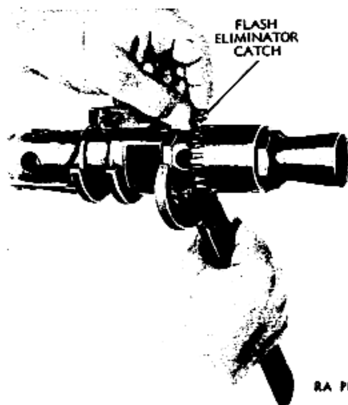
Figure 53 — Removal of Blast Trap and Flash Eliminator
