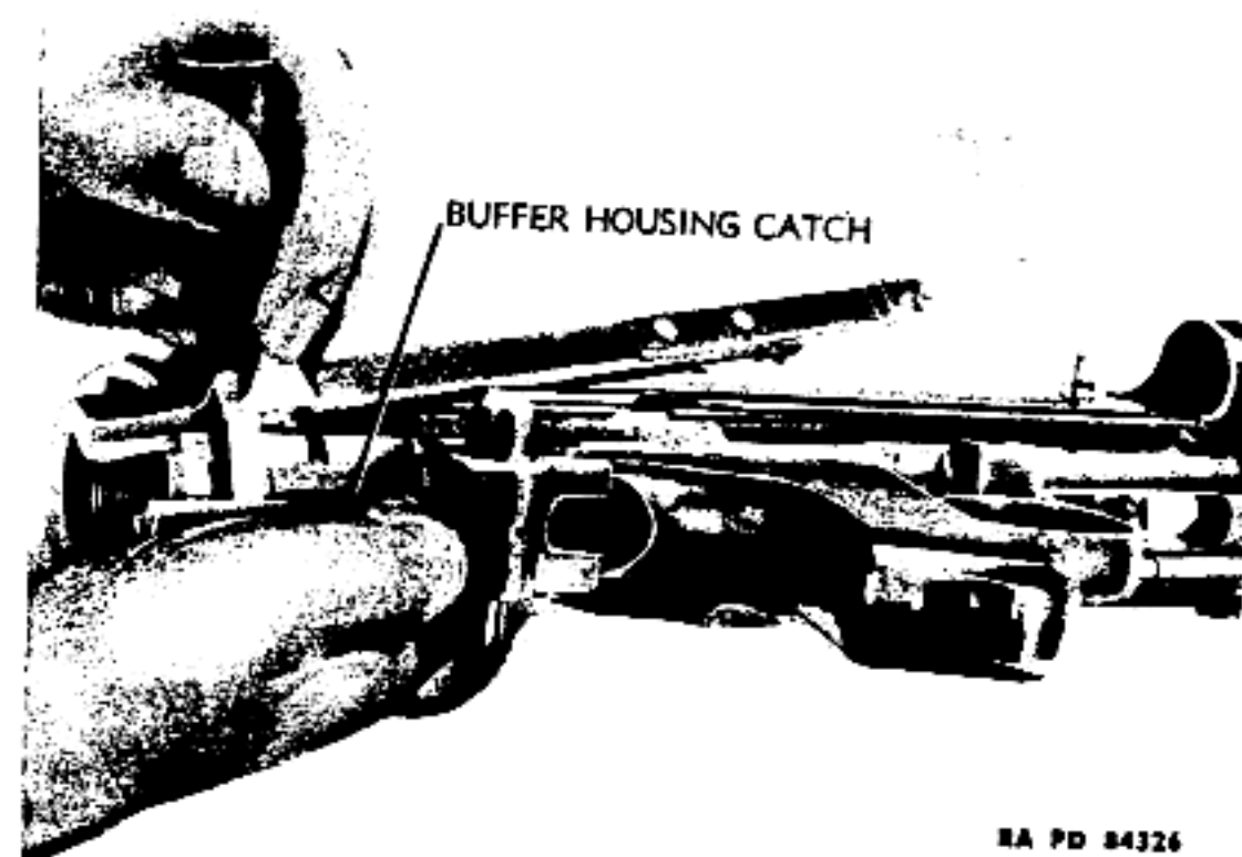
Figure 50 — Removal of Cocking Handle
