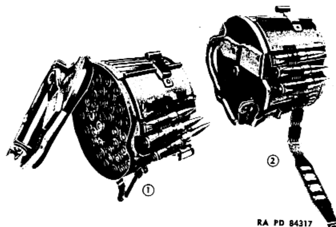
Figure 13 — Loading a Belt Drum Magazine
