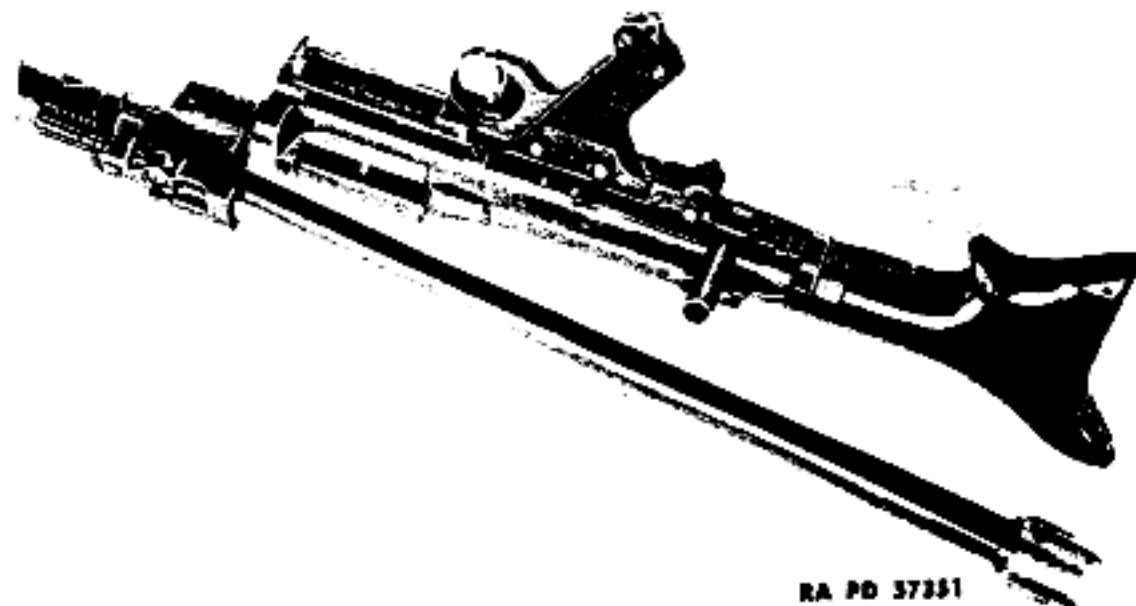
Figure 40 — Sliding Barrel out of Barrel Casing
