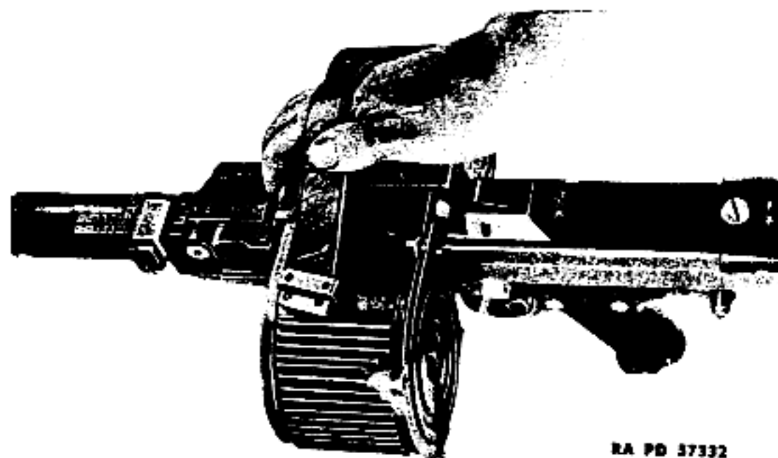
Figure 38 — Removal of 75-round Magazine
