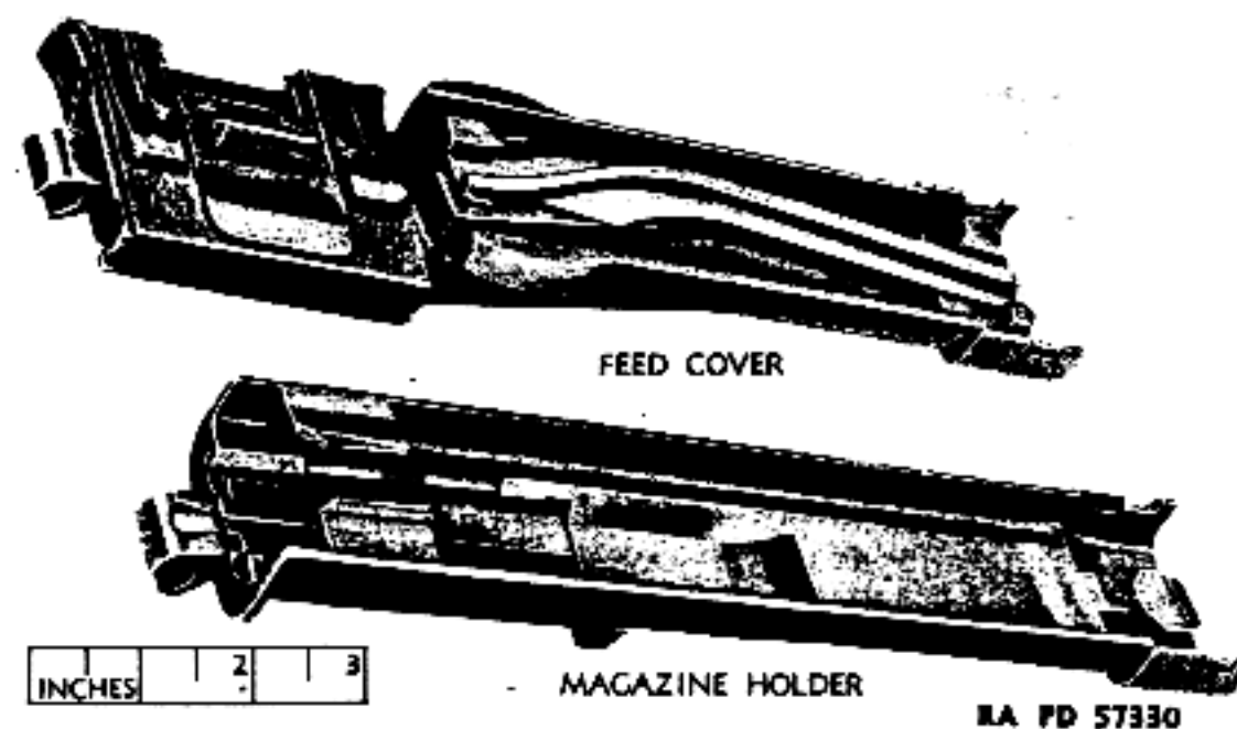
Figure 24 — Feed Cover and Magazine Holder — Bottom View
