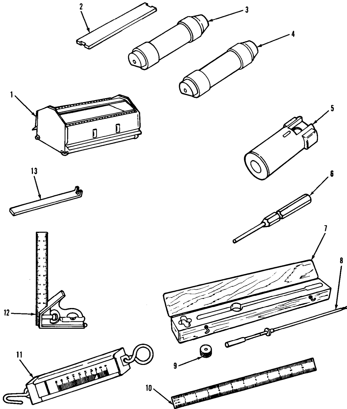
Figure 36. Special tools.
