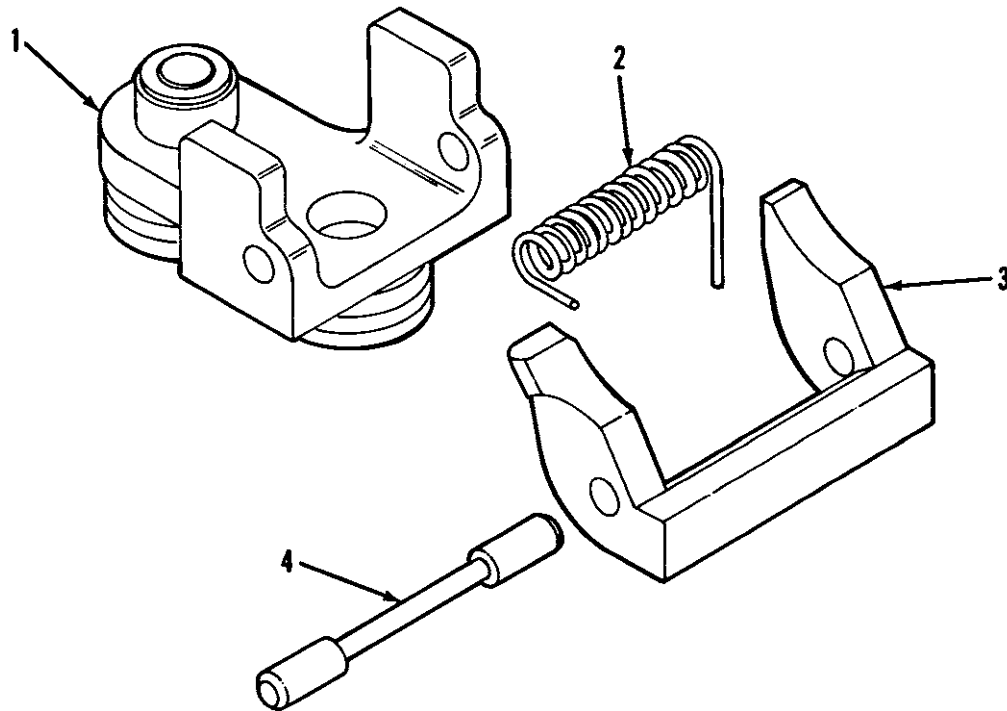
Figure 17. Feed pawl assembly.
