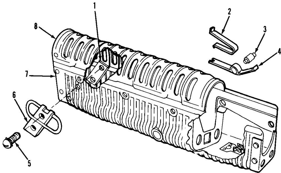
Figure 22. Forearm Assembly.
