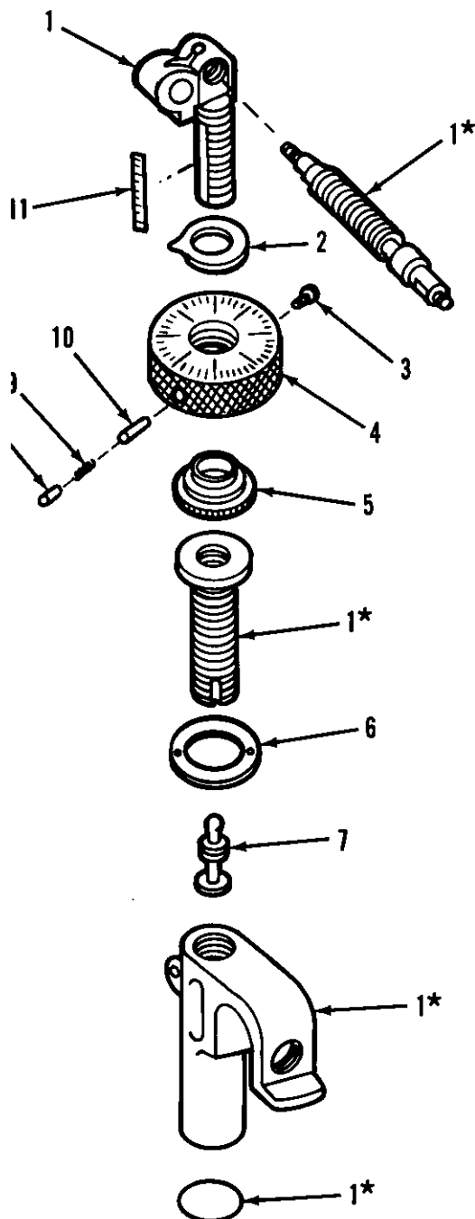
Figure 32. Traversing and elevating mechanism assembly (elevating unit).
