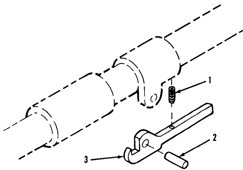
Figure 34. Tripod mount leg.
