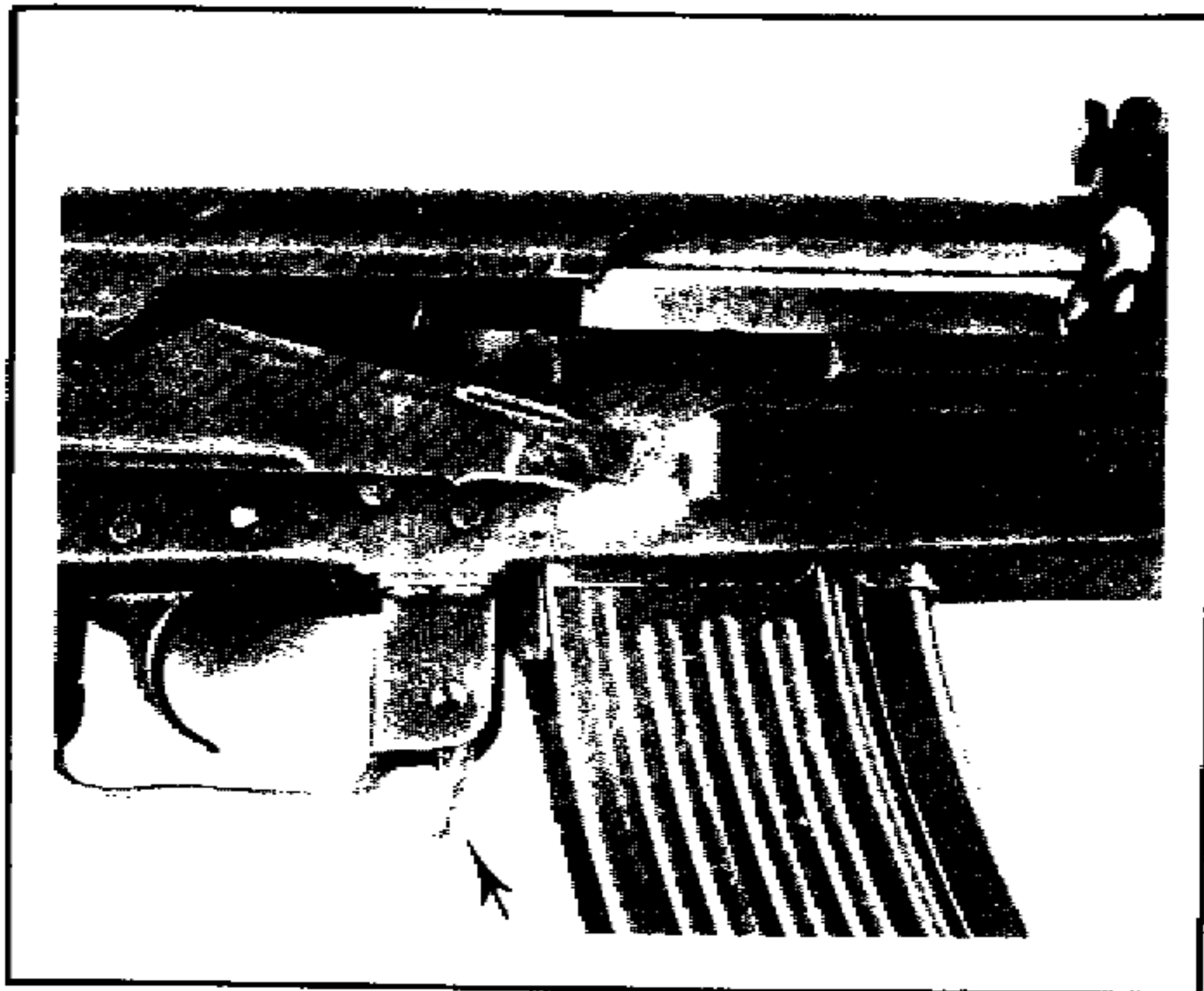
FIGURE 15. MAGAZINE CATCH
