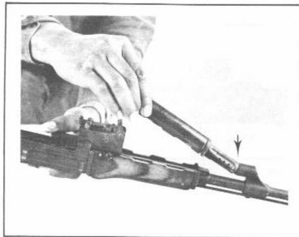
FIGURE 35. ENGAGING TUBE
