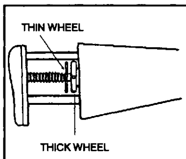
Figure 2-7. Stock adjustment.
